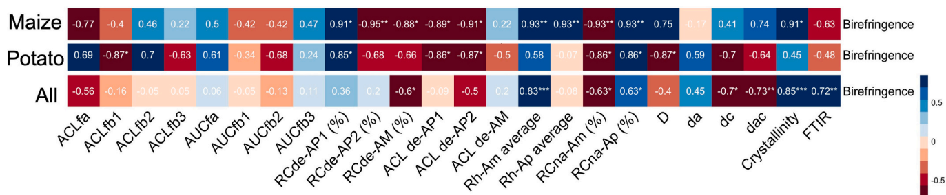
Fig. 3. The correlation between birefringence from the microscopy and starch structural parameters. RC_{de-x} : relative amount of fraction X of debranched sample; RC_{na-x} : relative amount of fraction X of native sample; ACL_{de-x} : the average chain length (DP) of the fraction X of debranched sample; Rh_{na-x} : hydrodynamic radius of fraction X of native sample. RC_x : relative amount of fraction X of debranched samples; ACL_x : average chain lengths (DP) of fraction X of debranched samples; fa: amylopectin chains with DP 6–12; fb1: amylopectin chains with DP 13–24; fb2: amylopectin chains with DP 25–36; fb3: amylopectin chains with DP >36. D, Bragg lamellar repeat distance; d_{ac} , d_a and d_c , the thicknesses of total, amorphous, and crystalline lamellae, respectively; FTIR: the ratio of 1045/1022 cm^{-1} . *, **, and *** indicate significant correlations at p < 0.05 , 0.01, and 0.001 levels, respectively.
